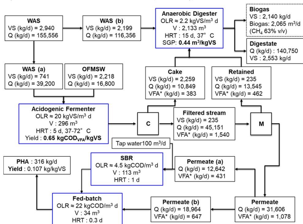
Figure 1: Mass balance of the whole biorefinery technology chain.
