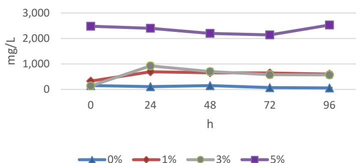
Figure 3: COD concentration in effluent within 96 h at different microbe dosing (1 %, 3 % and 5 %) compared to the control (0% - no microbe dosing)
